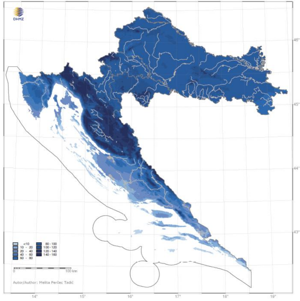
Srednji godišnji broj hladnih dana ( t_{\text{min}} < 0^{\circ}\text{C} ) Mean annual number of frost days ( t_{\text{min}} < 0^{\circ}\text{C} )
