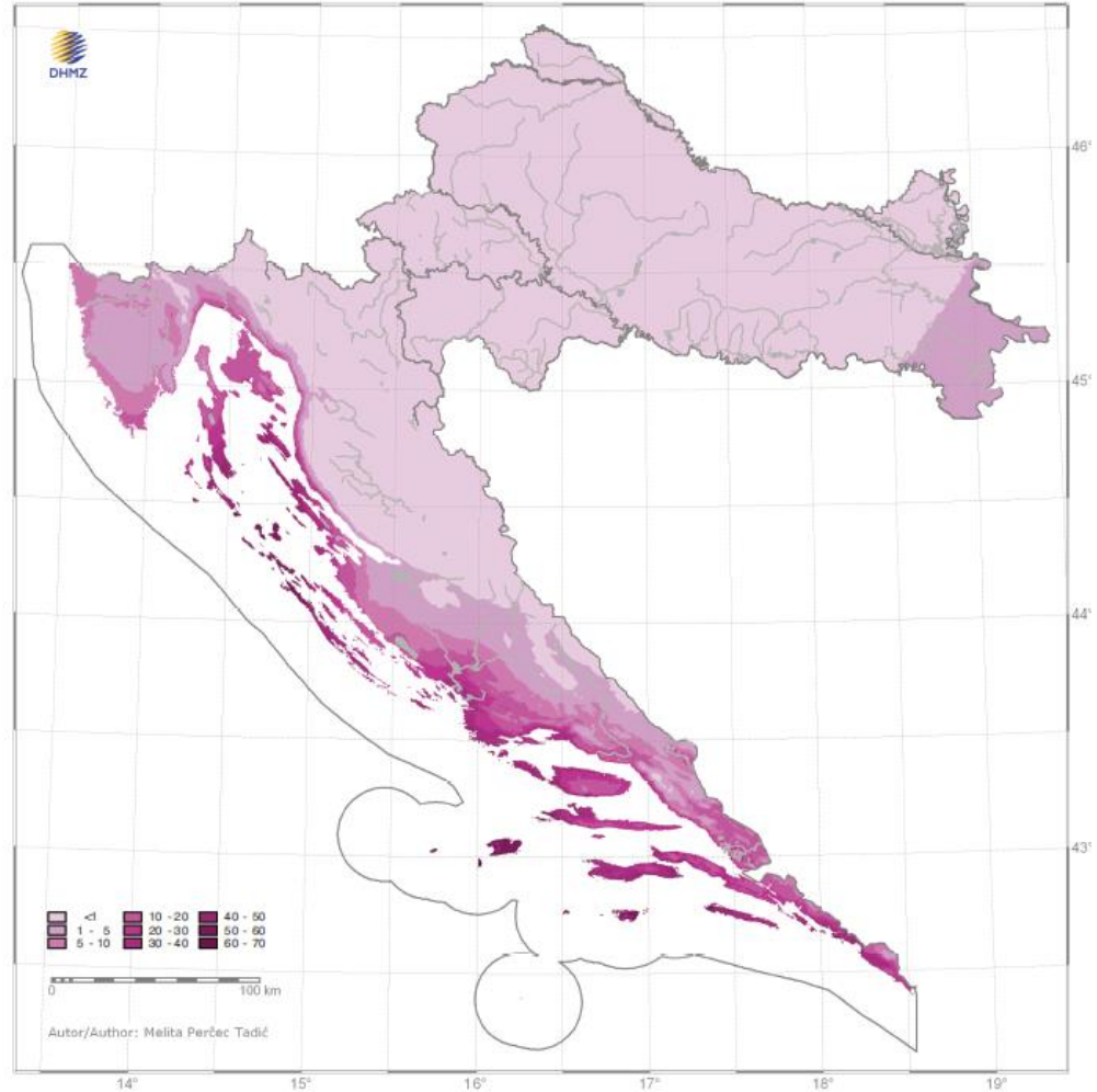
Srednji godišnji broj toplih noći ( t_{\min} \geq 20^\circ\text{C} ) Mean annual number of tropical nights ( t_{\min} \geq 20^\circ\text{C} )
